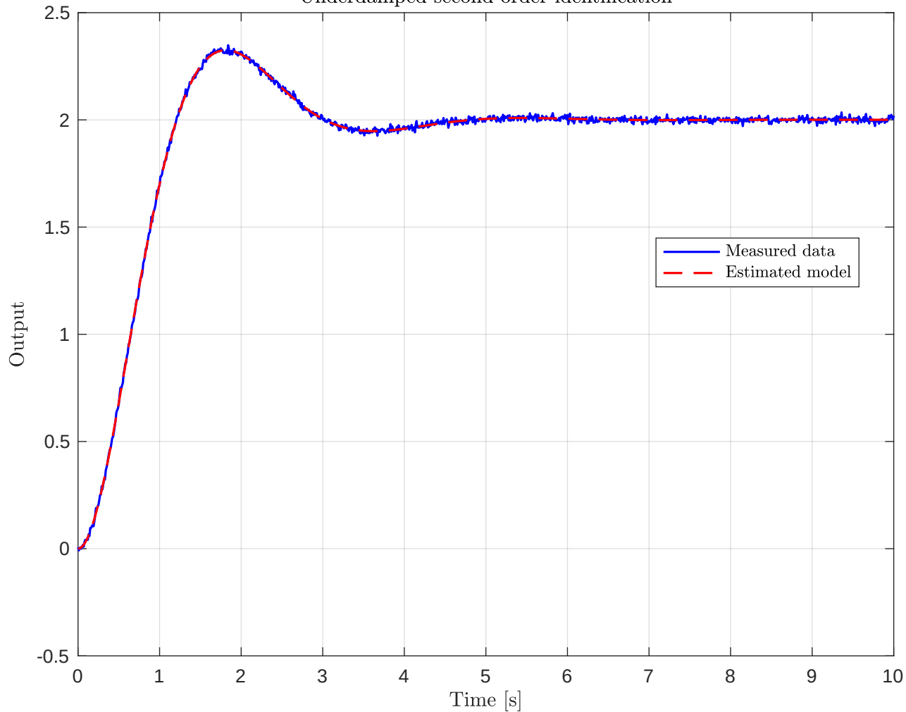
Underdamped second-order identification
