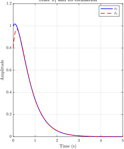
State x_1 and its estimation
