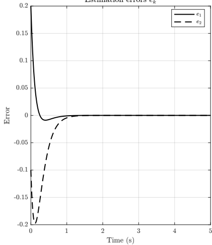
Estimation errors e_k
