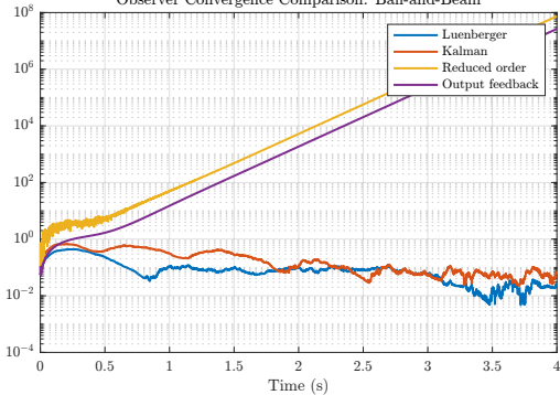
Observer Convergence Comparison: Ball-and-Beam
