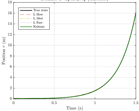
Scenario 1: Open-Loop (Unstable)
