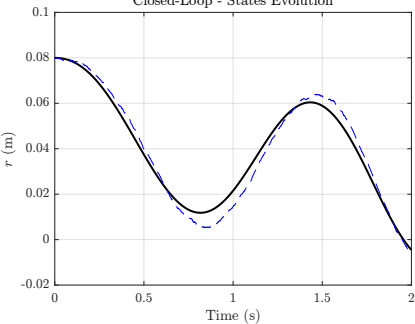
Closed-Loop - States Evolution
