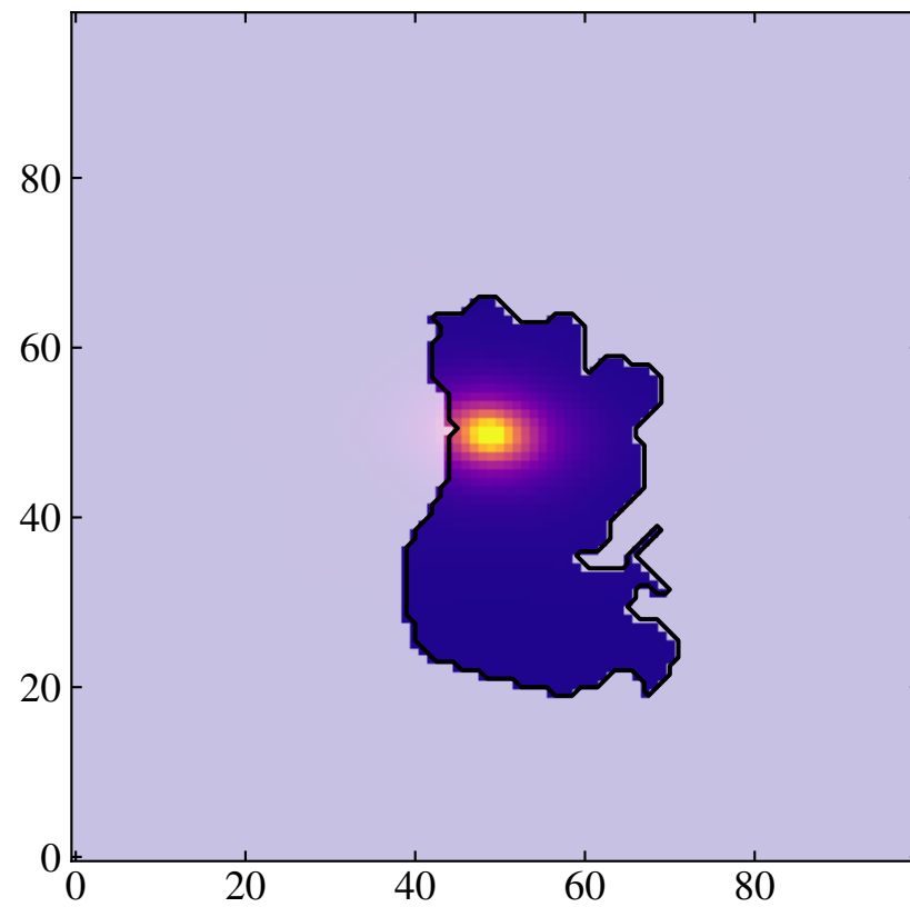
Model
