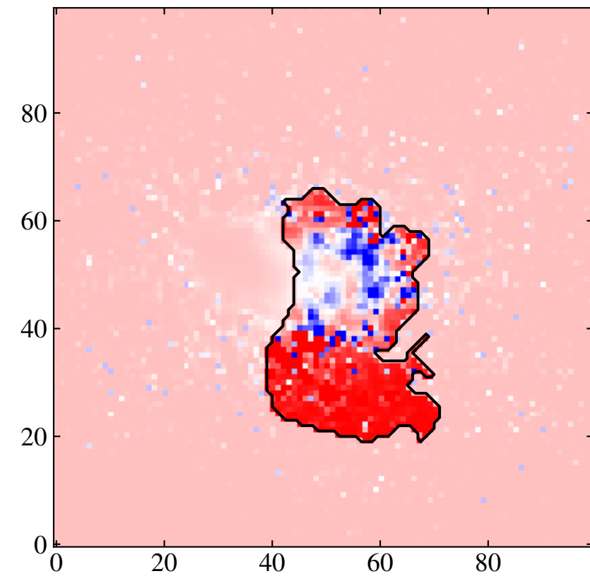
Residuals
