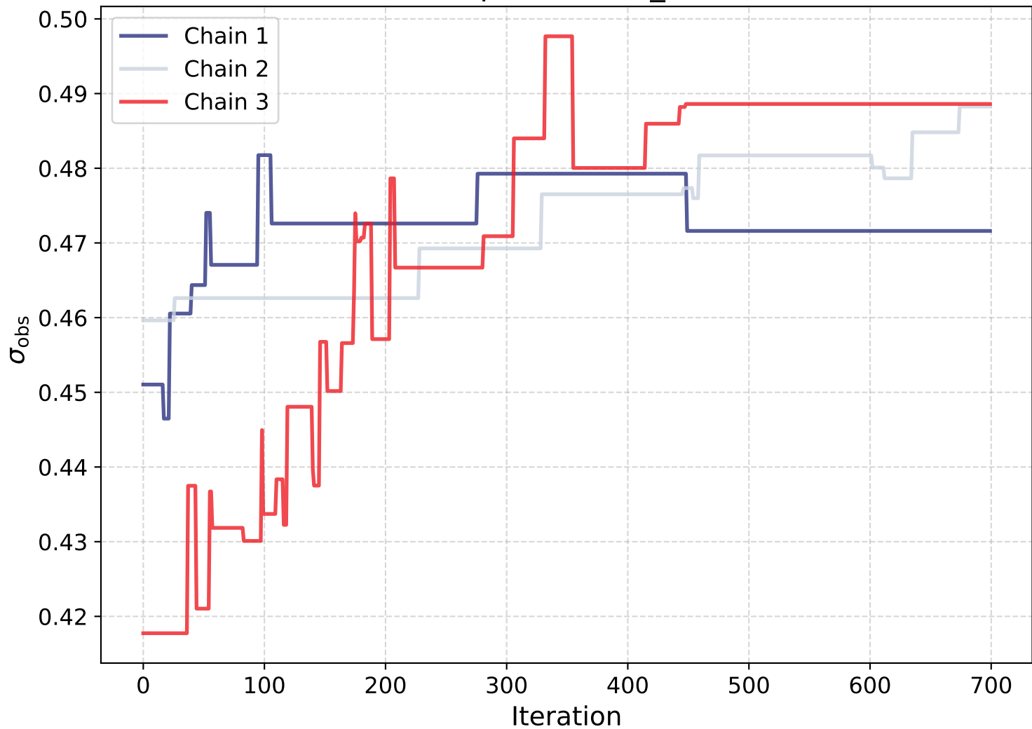
Trace plot for obs_scale
