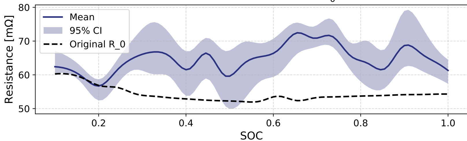
Posterior Distribution of R'_0
