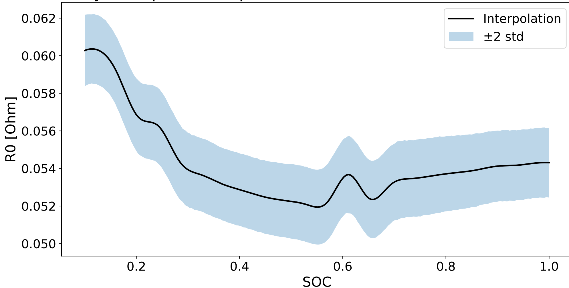
Uncertainty in R0 prediction (prior distribution) with constant variance of 1e-06
