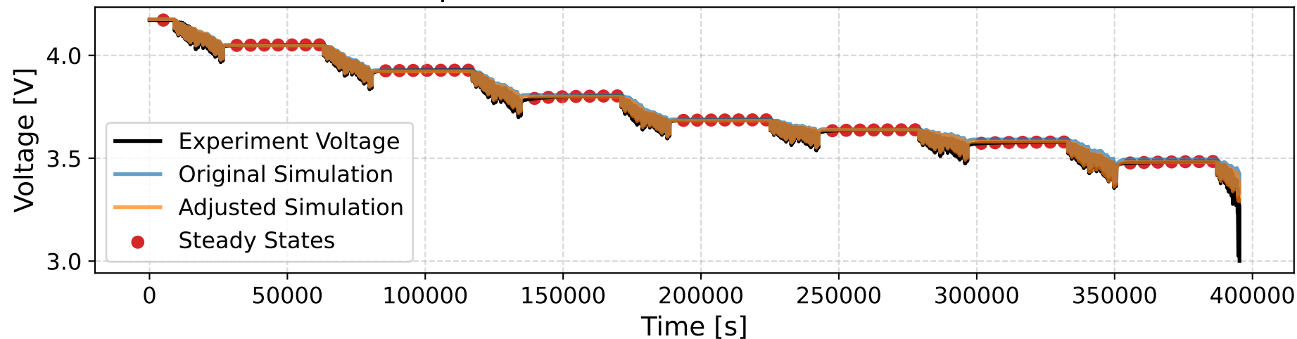
Experiment Data vs Simulation Results
