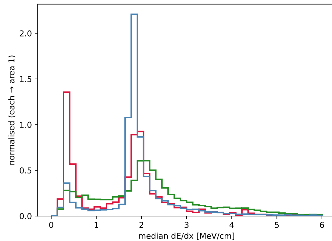
CNN: what makes \gamma look like \pi^\pm ?
