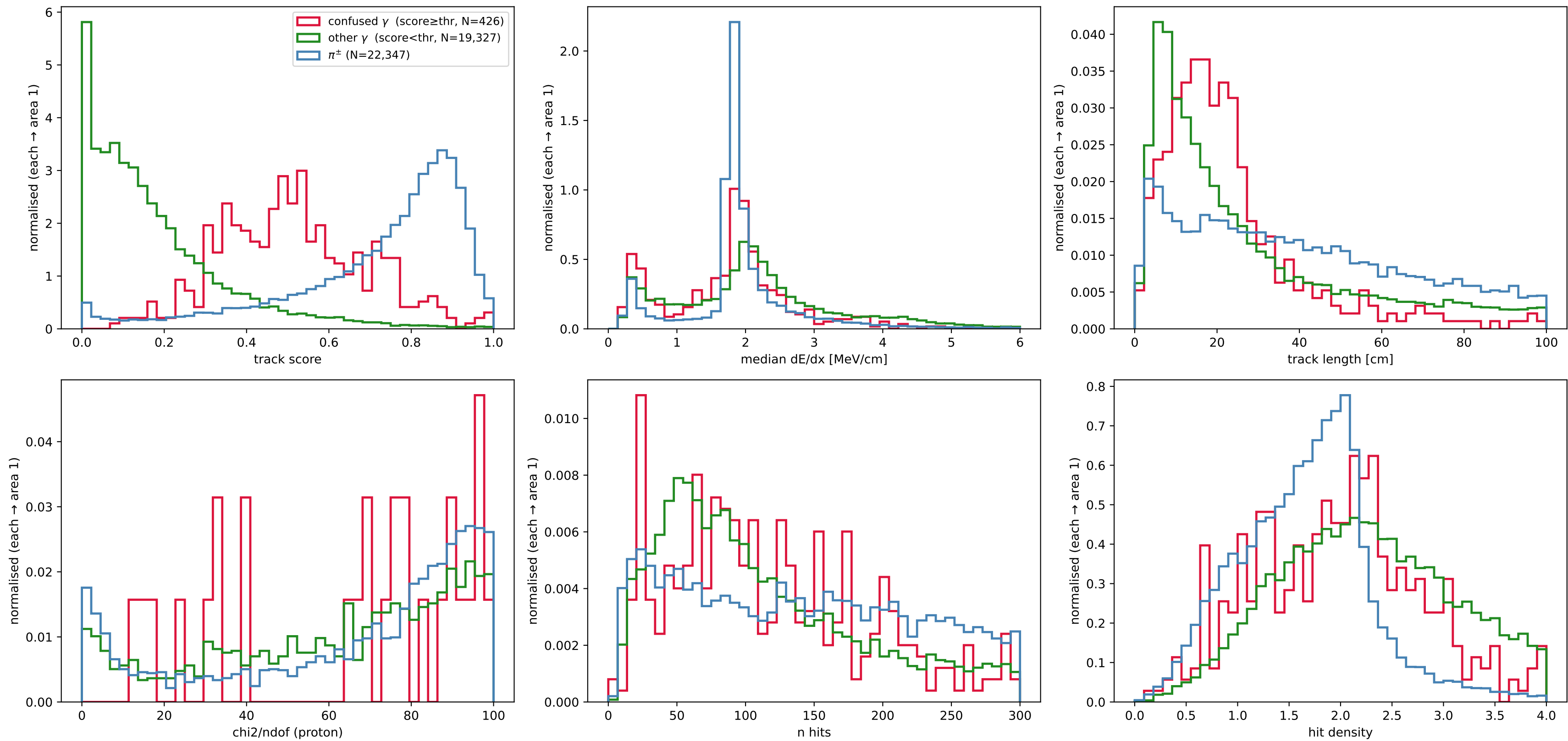
Hybrid all8: what makes \gamma look like \pi^\pm ?
