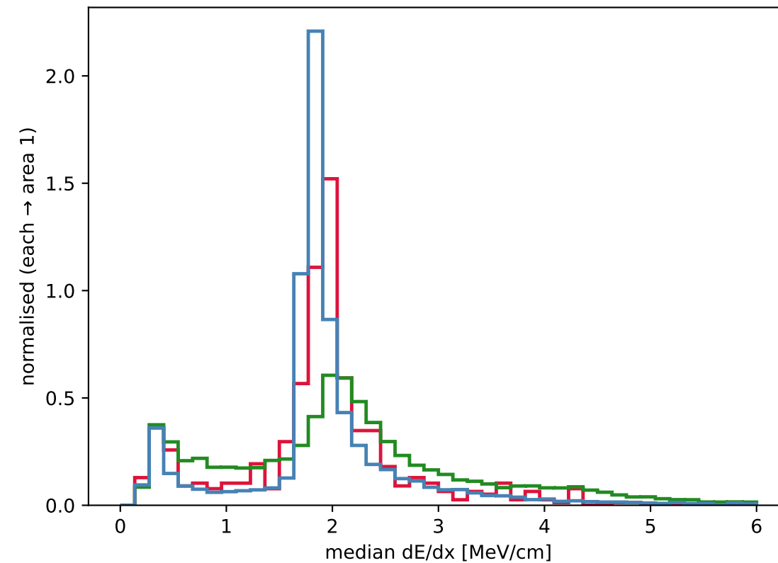
Hybrid: what makes \gamma look like \pi^\pm ?
