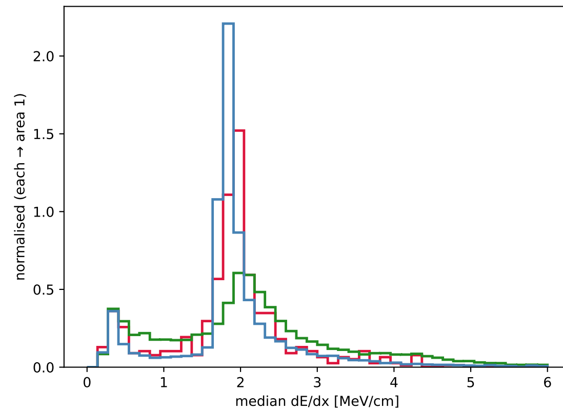
Hybrid base4: what makes \gamma look like \pi^\pm ?
