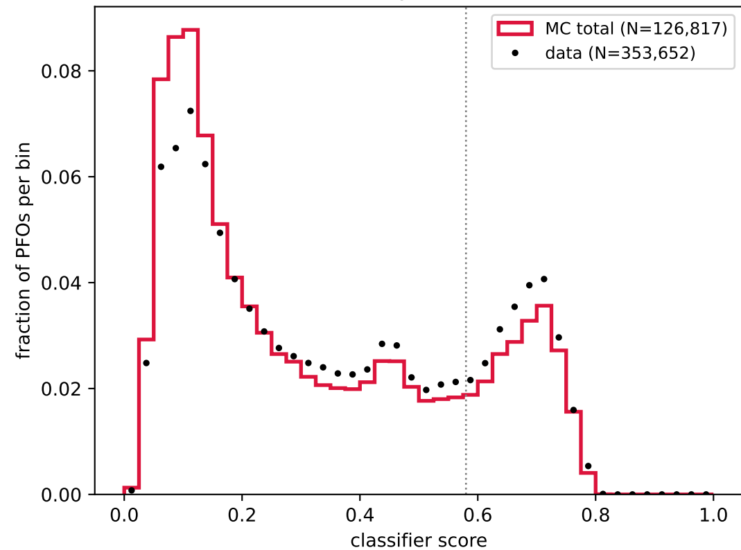
Hybrid
