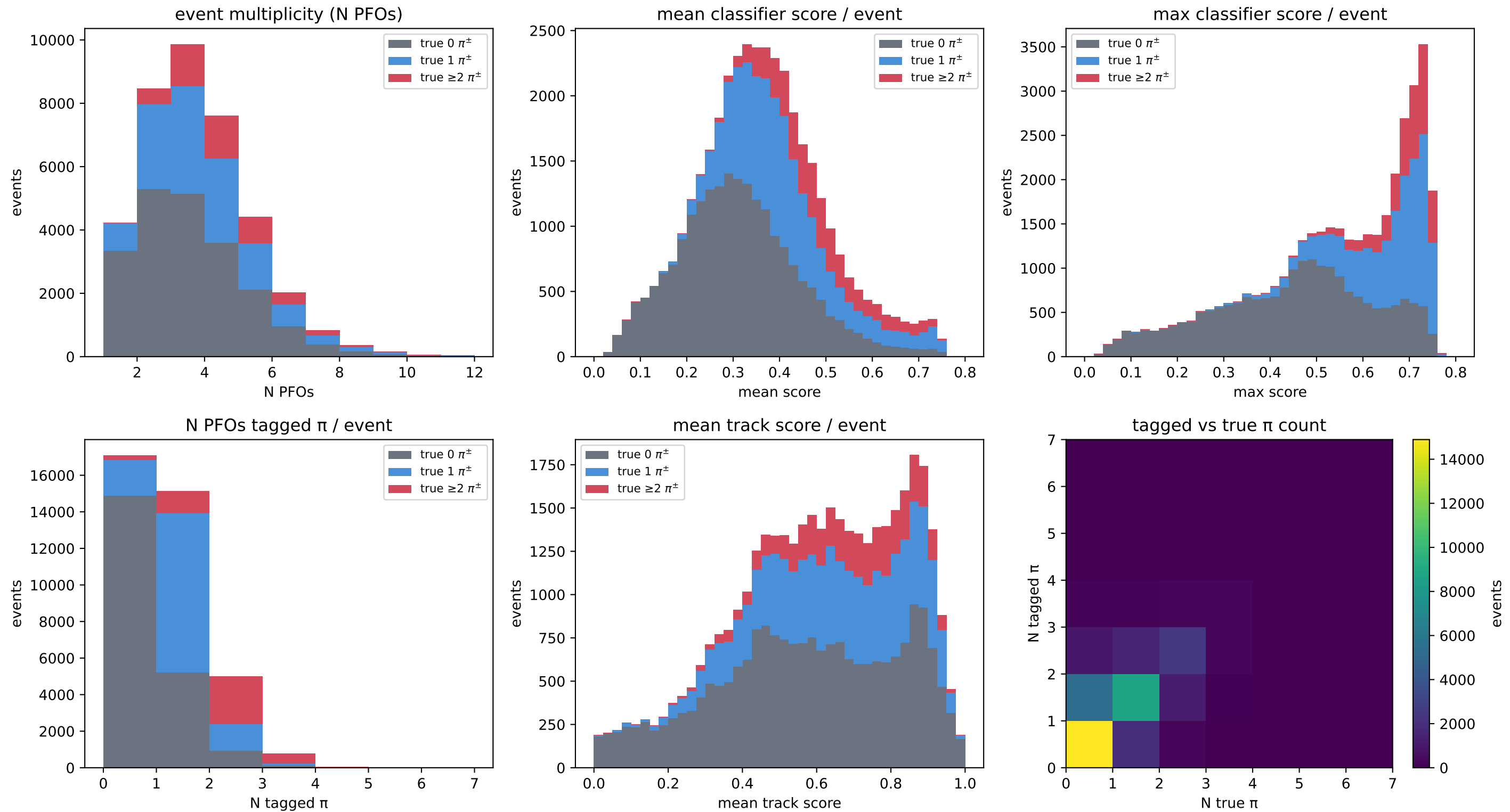
Hybrid: event-level observables (MC test) — colour = true \pi -count bin
