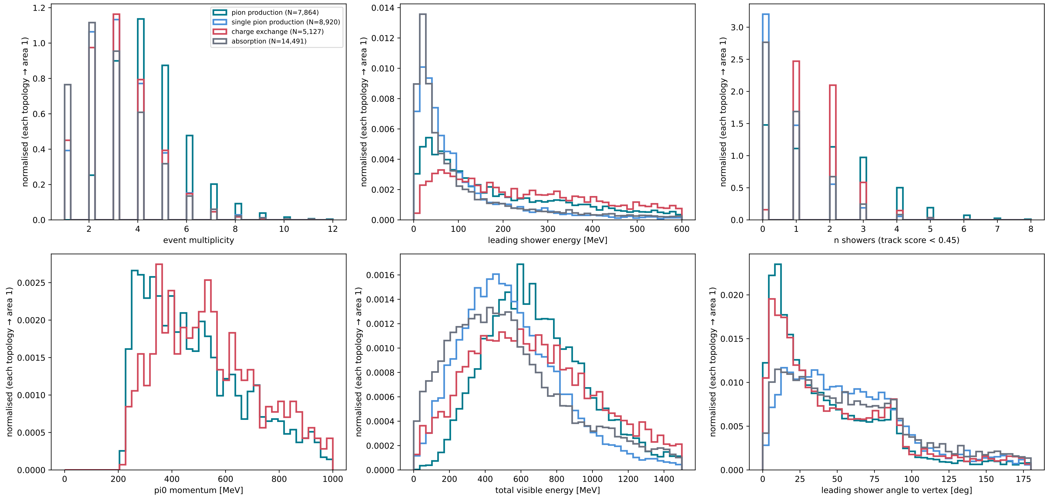
Best-separating geometric observables, by true FSI topology
