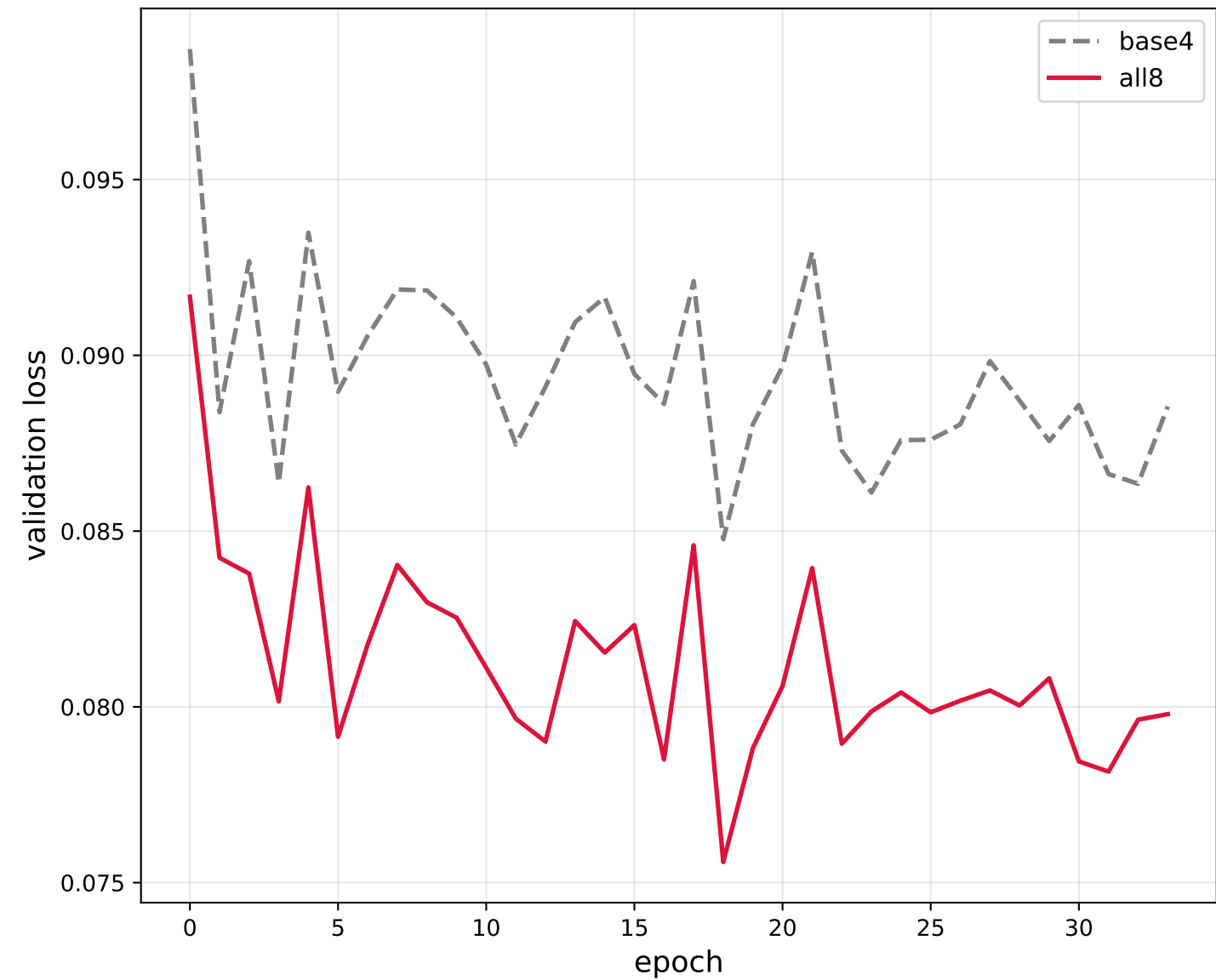
Validation loss
