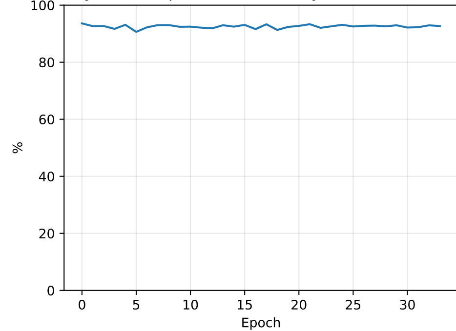
Hybrid all8 (photon) - Efficiency (threshold=0.5)
