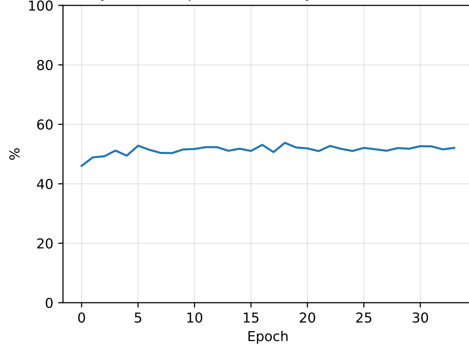
Hybrid all8 (photon) - Purity (threshold=0.5)
