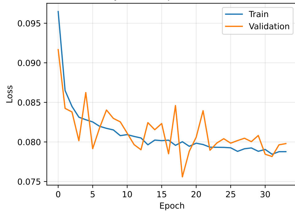
Hybrid all8 (photon) - Loss
