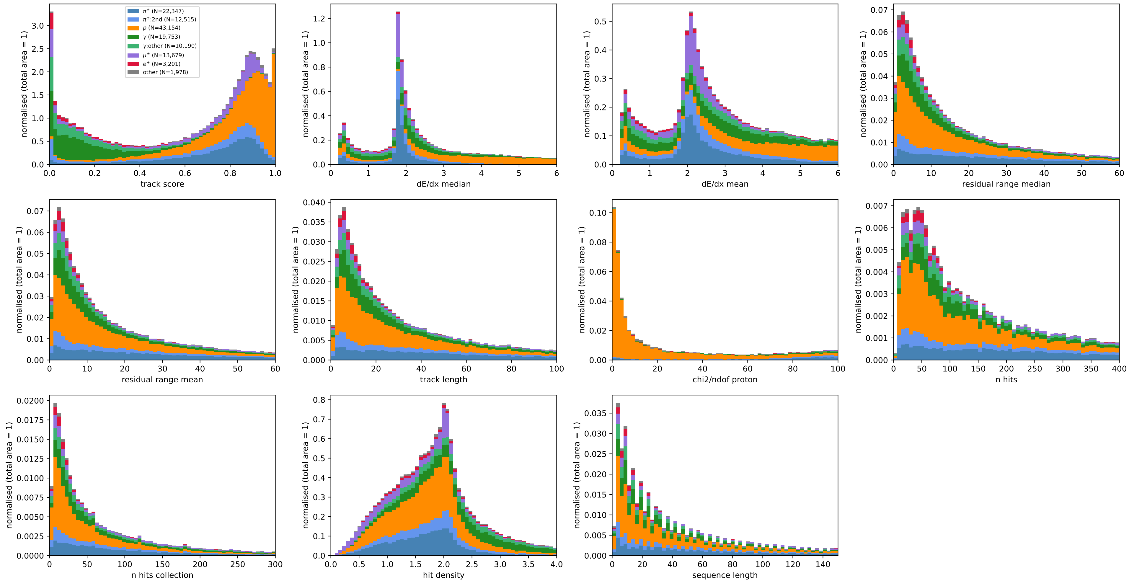
Observables before classification — stacked by species, total N = 126,817
