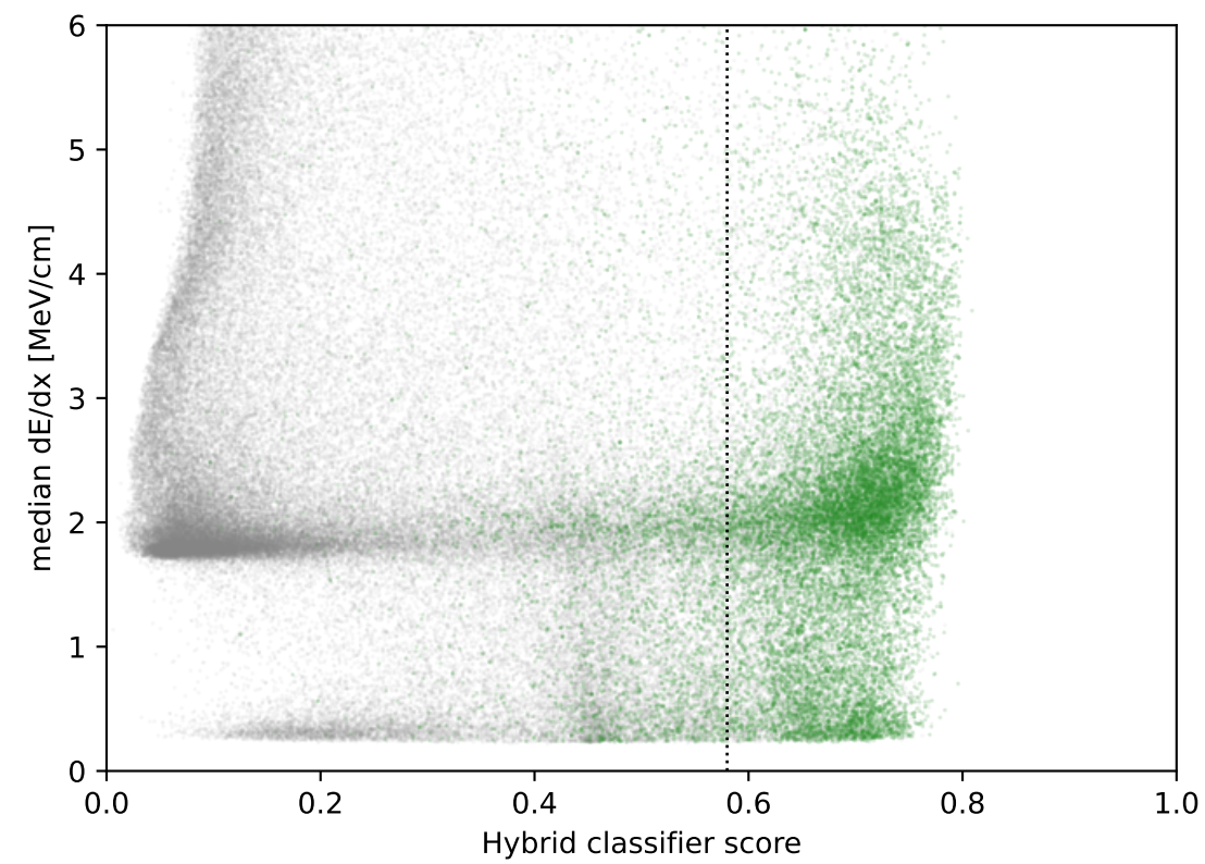
Hybrid: observables vs score ( \gamma (beam \pi^0 ) vs background)
