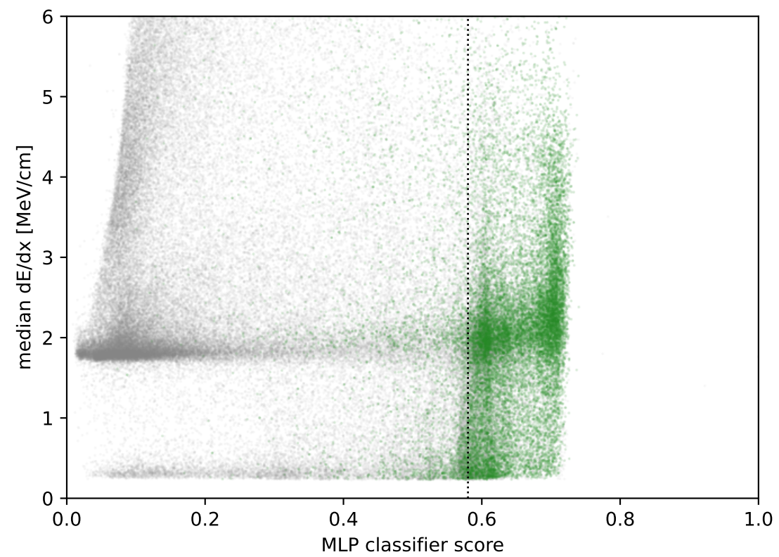
MLP: observables vs score ( \gamma (beam \pi^0 ) vs background)
