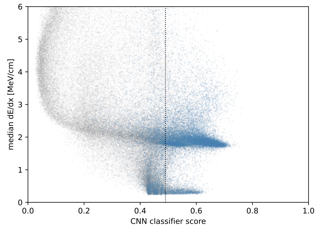
CNN: observables vs score ( \pi^\pm vs background)
