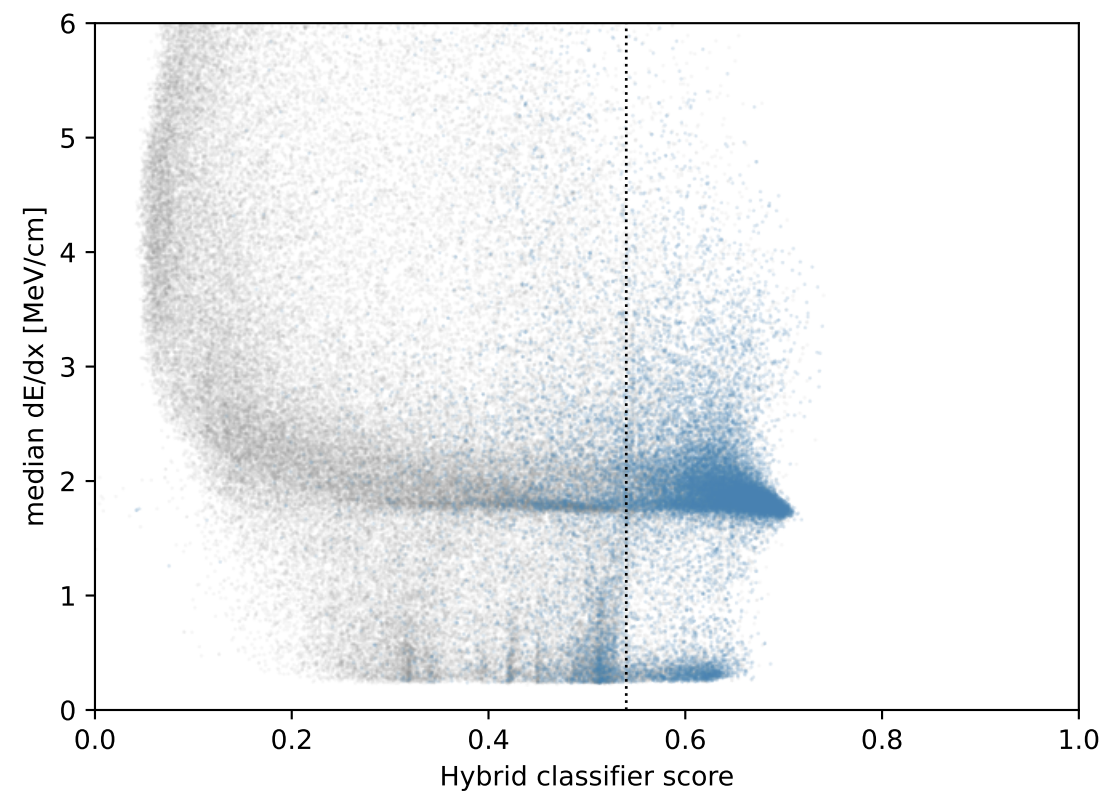
Hybrid: observables vs score ( \pi^\pm vs background)
