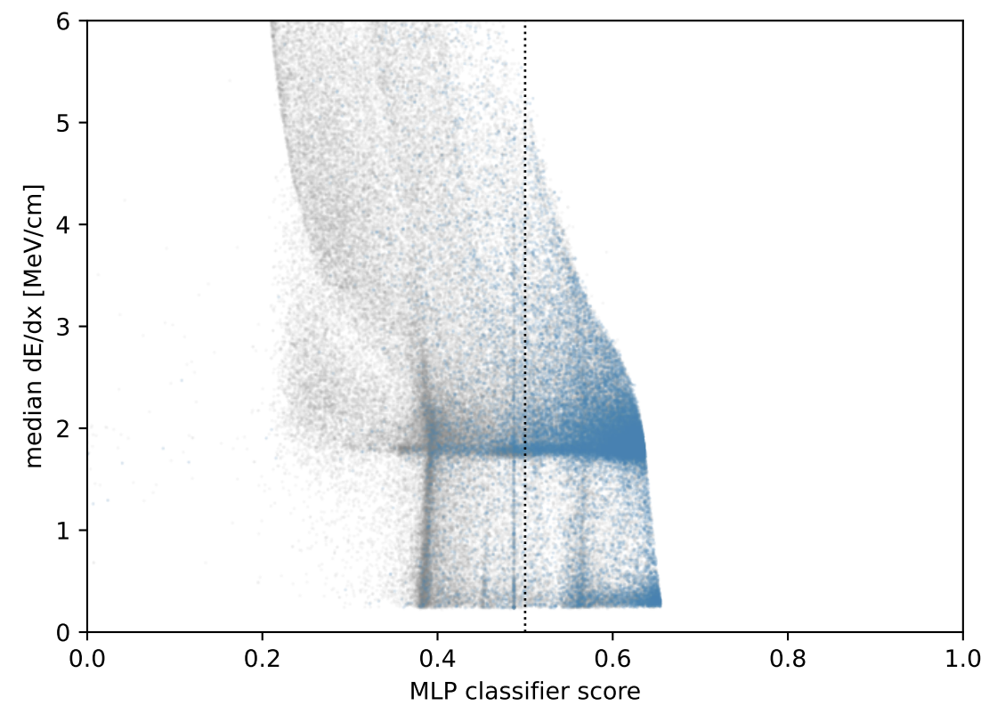
MLP: observables vs score ( \pi^\pm vs background)
