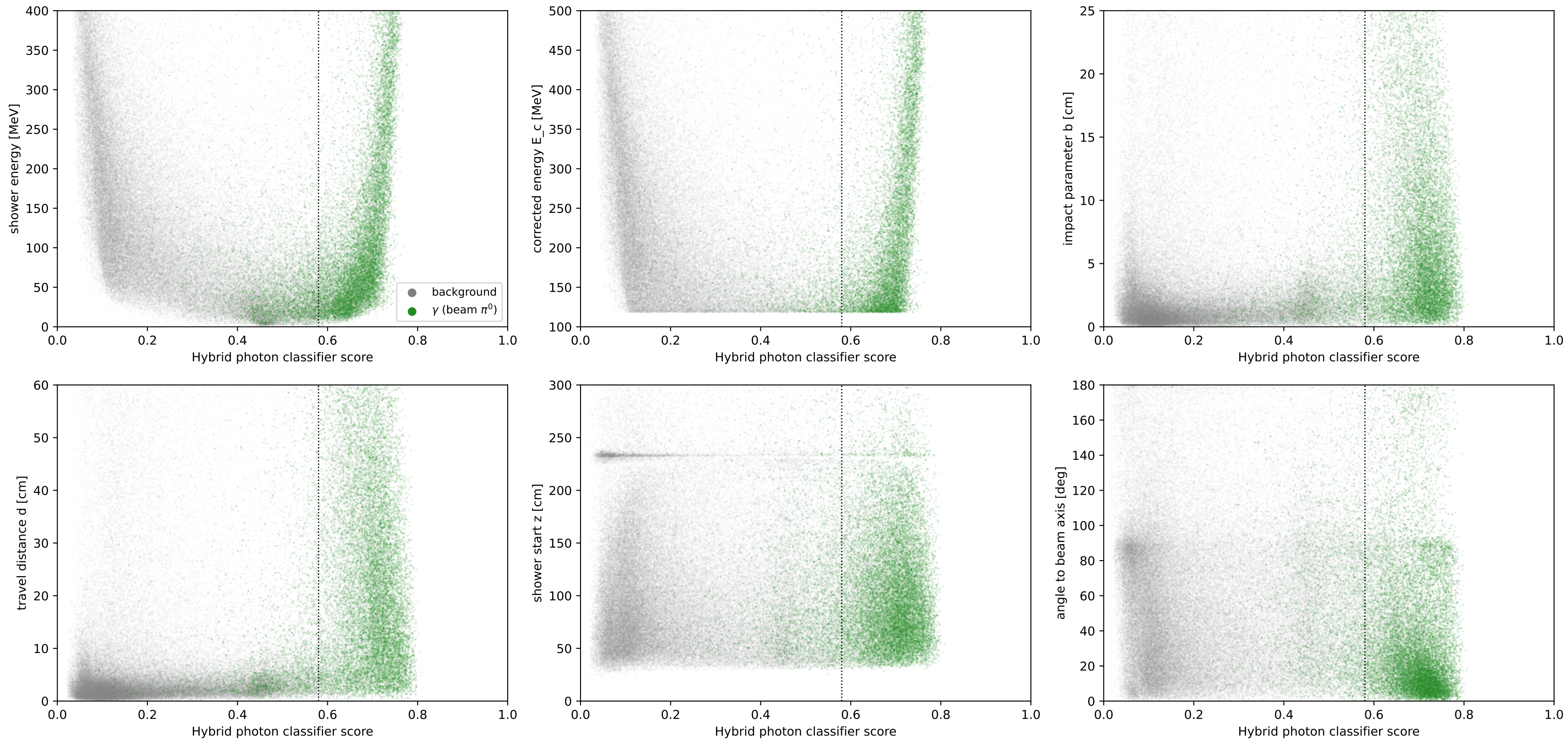
Shower observables vs classifier score
