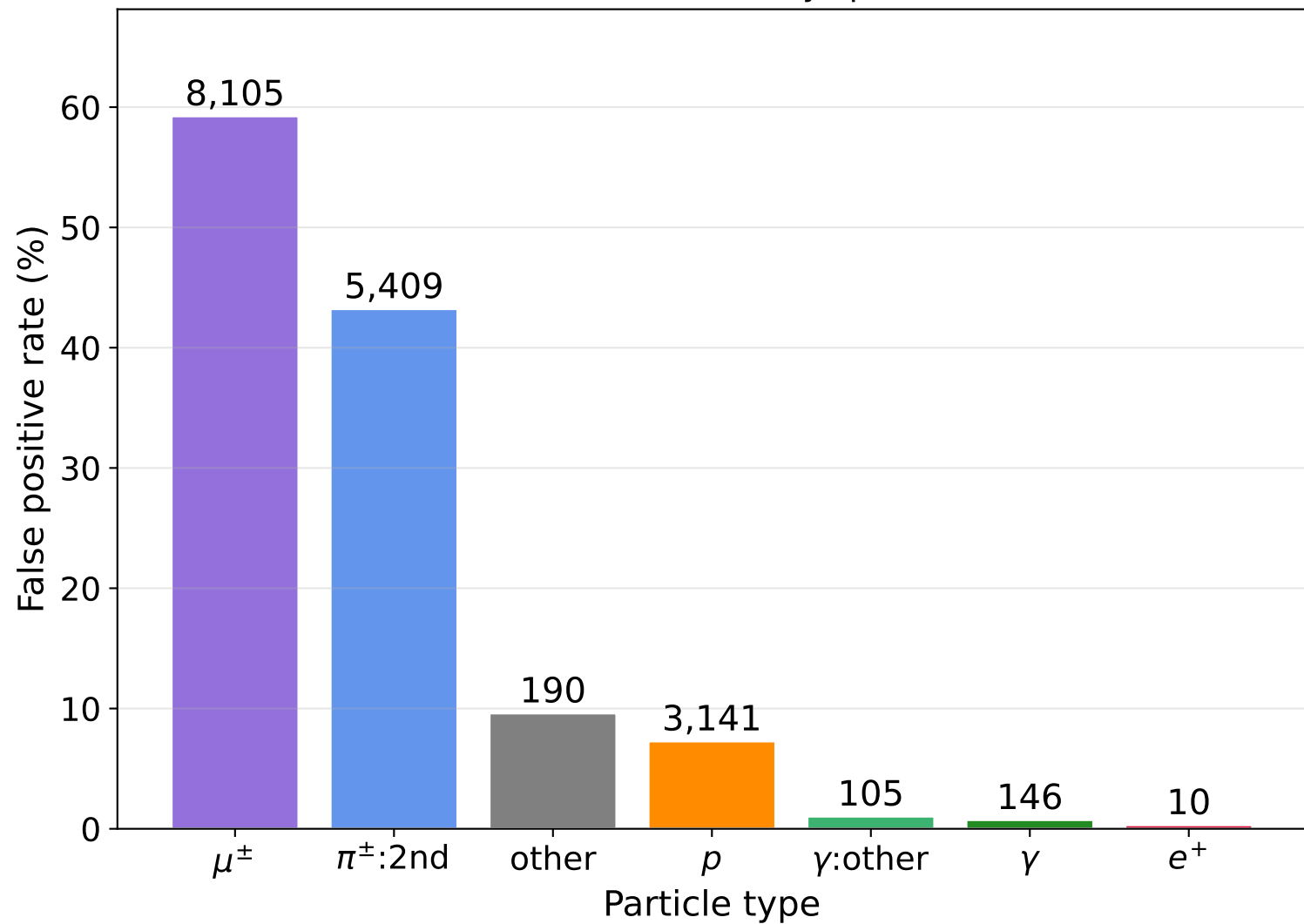
Cut-based \pi^\pm selection: FP rate by species (17,106 FPs)
