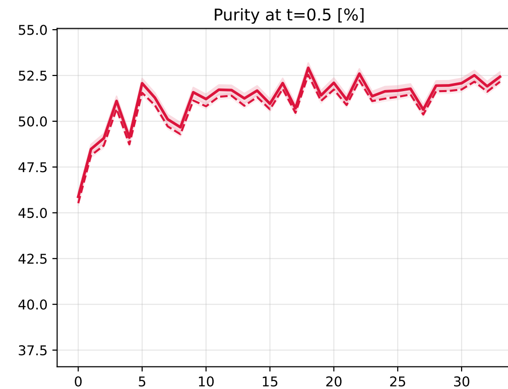
Train vs test by epoch — solid = test, dashed = train, shaded = binomial 1 \sigma
