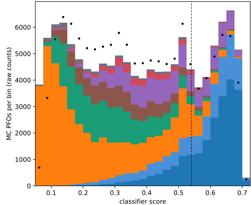
Hybrid
