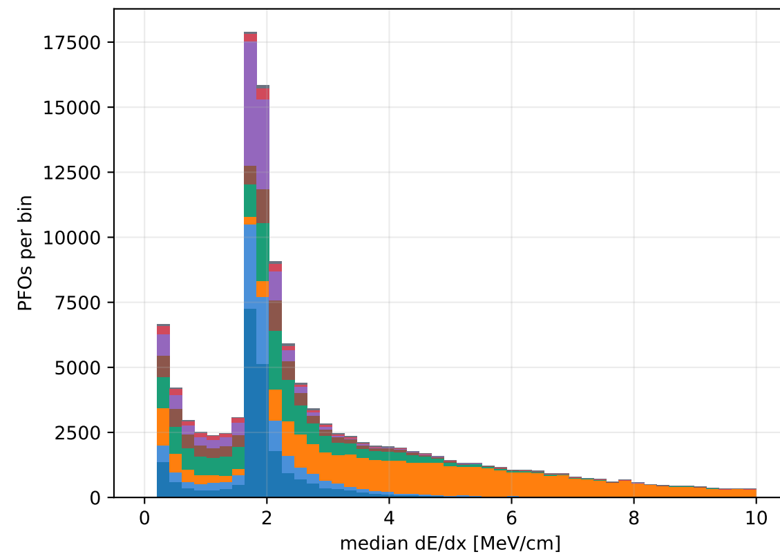
Input observables by true species — stacked, raw counts (N = 126,817)
