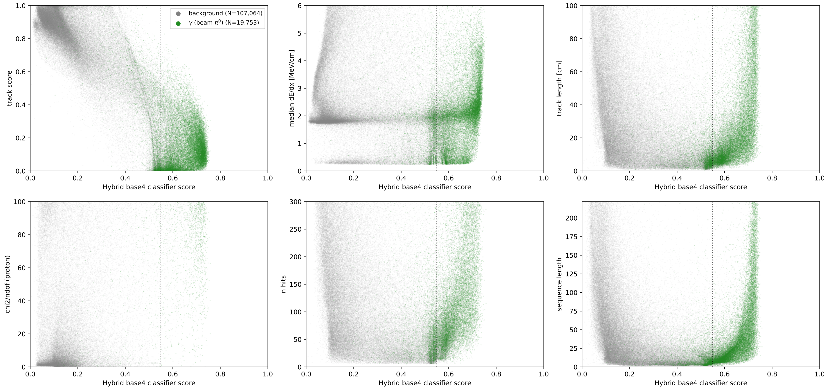
Hybrid base4: observables vs score ( \gamma (beam \pi^0 ) vs background)
