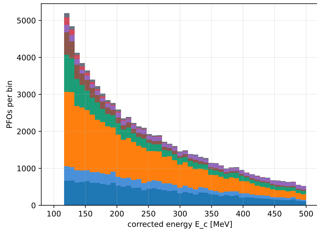
Shower observables by true species (MC test set)
