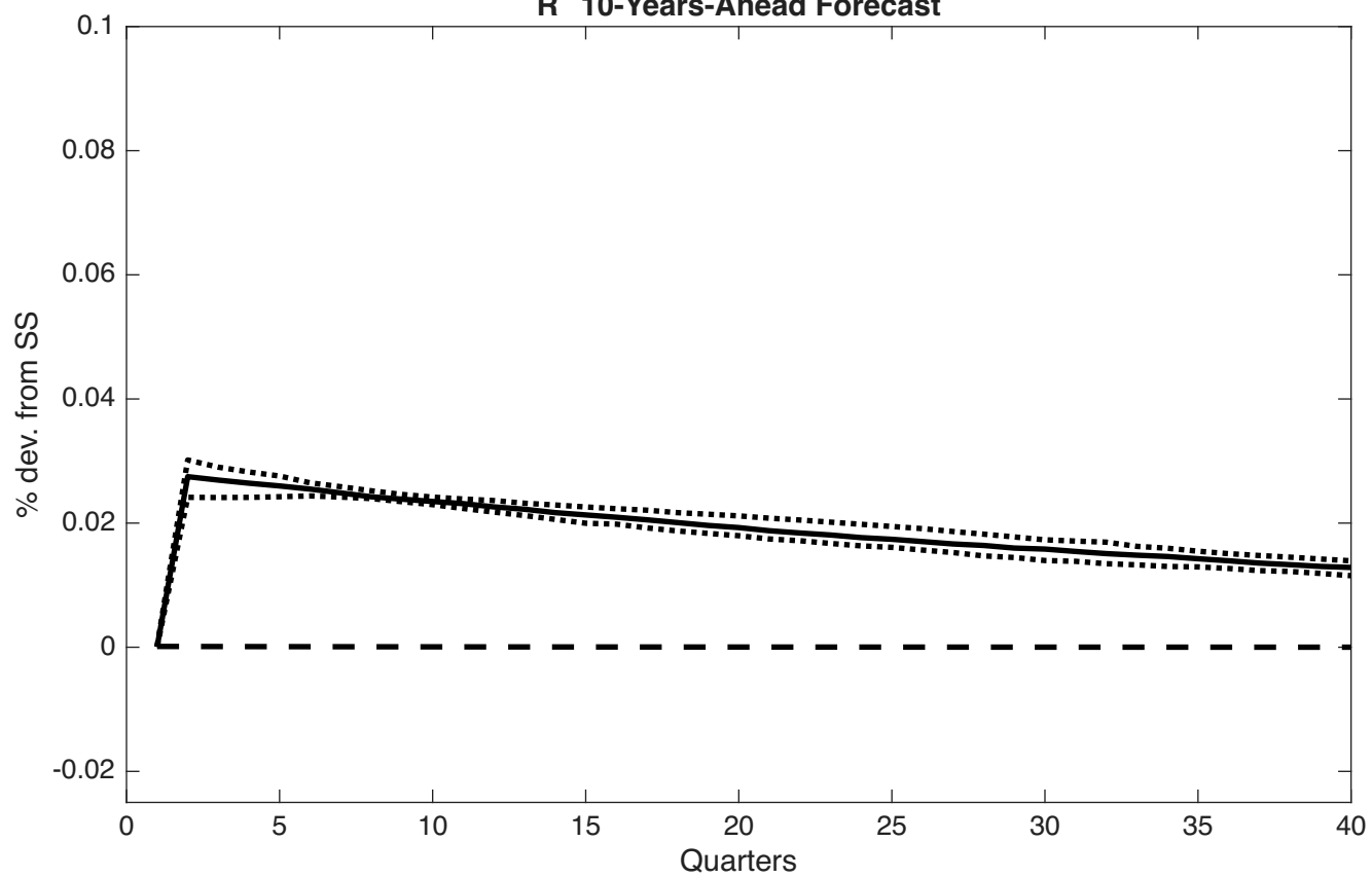
R^k 10-Years-Ahead Forecast
