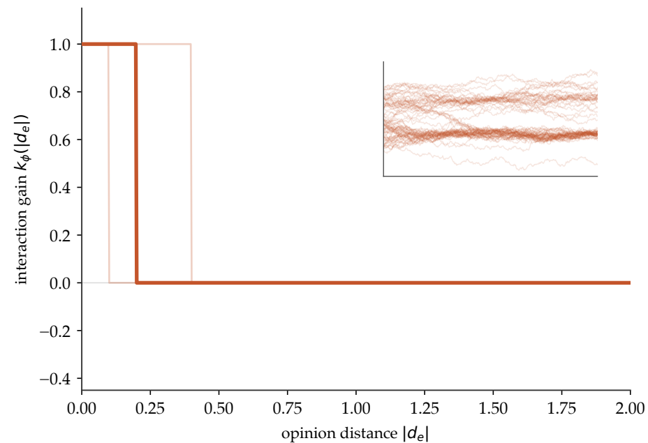
Bounded Confidence k_\phi(|d_e|) = \mathbf{1}_{\{|d_e| < \phi\}}
