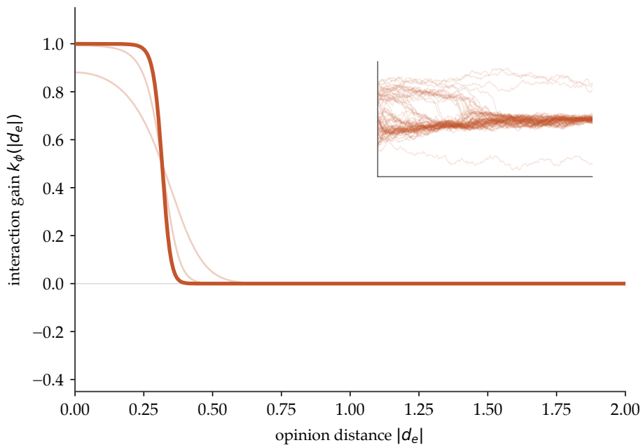
SAR k_\phi(|d_e|) = \left(1 - \frac{|d_e|^2}{\phi^2}\right) \exp\left(-\frac{|d_e|^2}{2\phi^2}\right)
