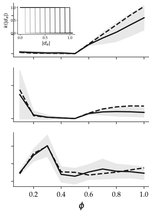
Bounded Confidence
