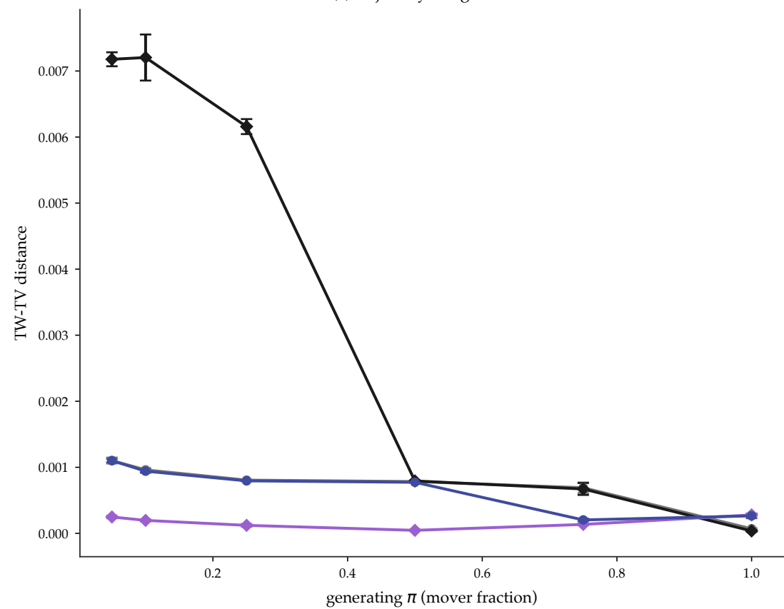
(c) trajectory-weighted TV
