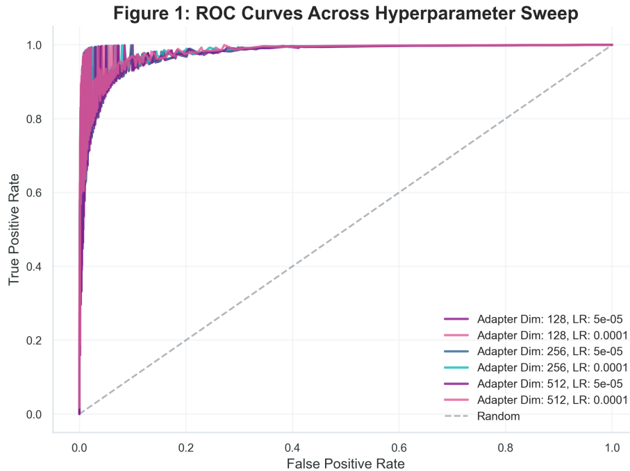
Figure 1: Figure 1: ROC Curves Across Hyperparameter Sweep. The curves demonstrate the robustness of BERT adapters across different bottleneck dimensions and learning rates. All configurations achieve an AUC > 0.92 , with the d = 512 configuration showing the fastest convergence.
