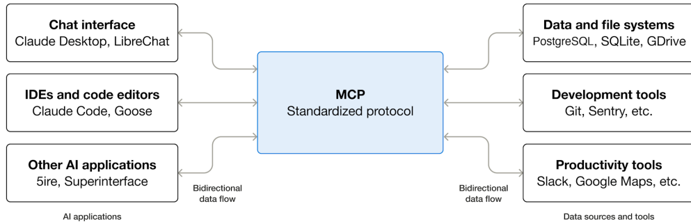
Figure 1: MCP Architecture
