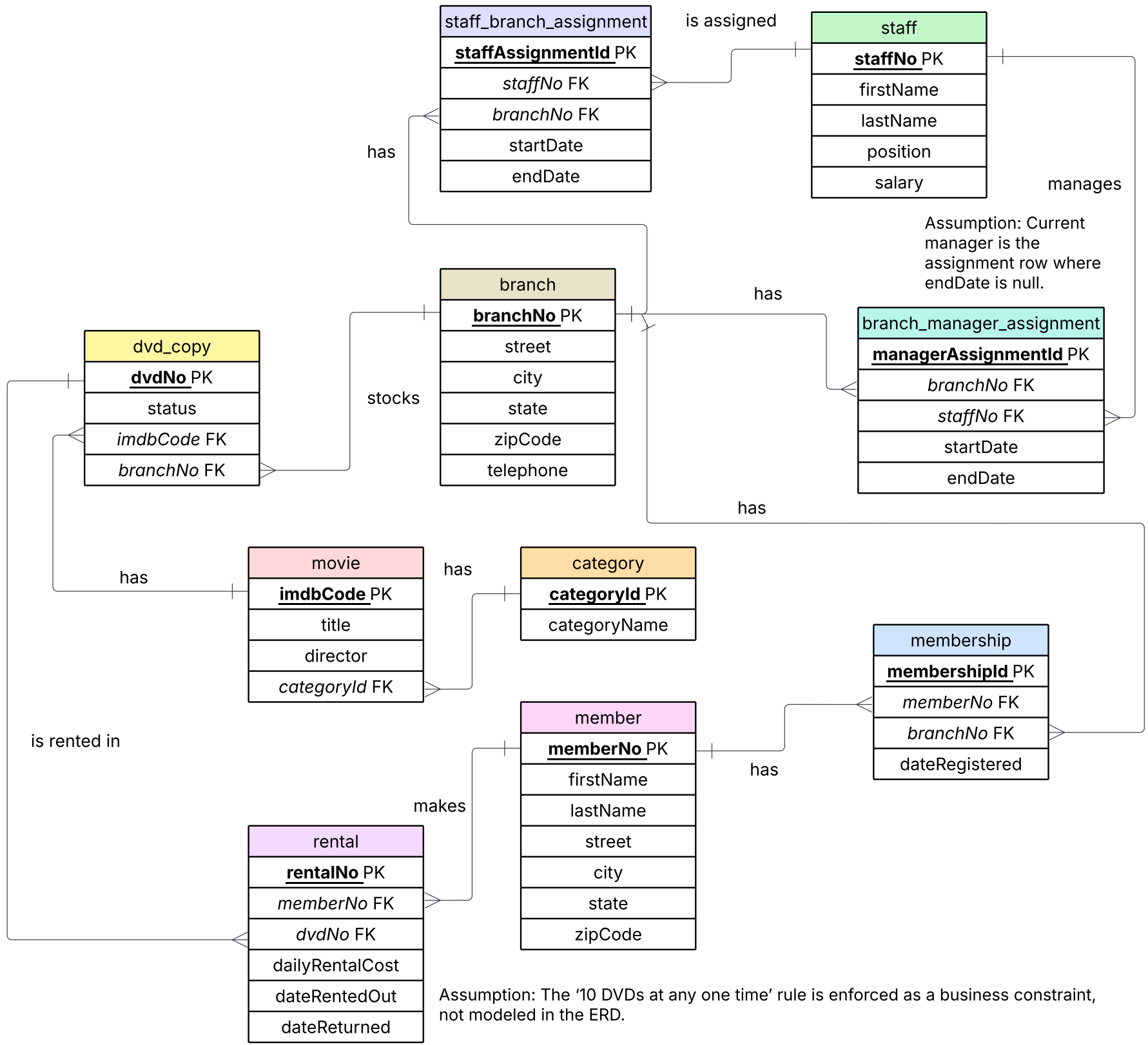
dvd_rental_company_erd
