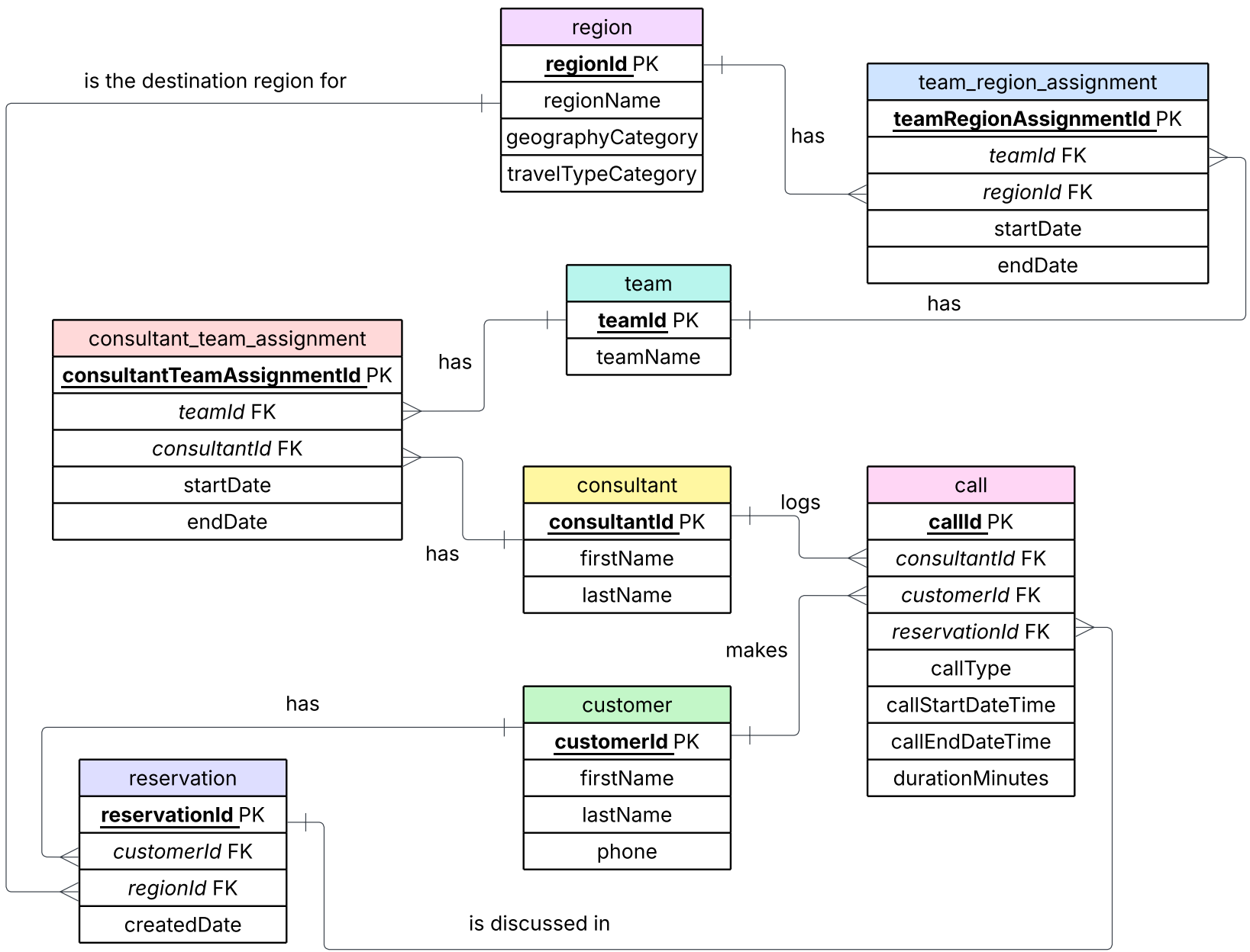
travel_consulting_company_erd
