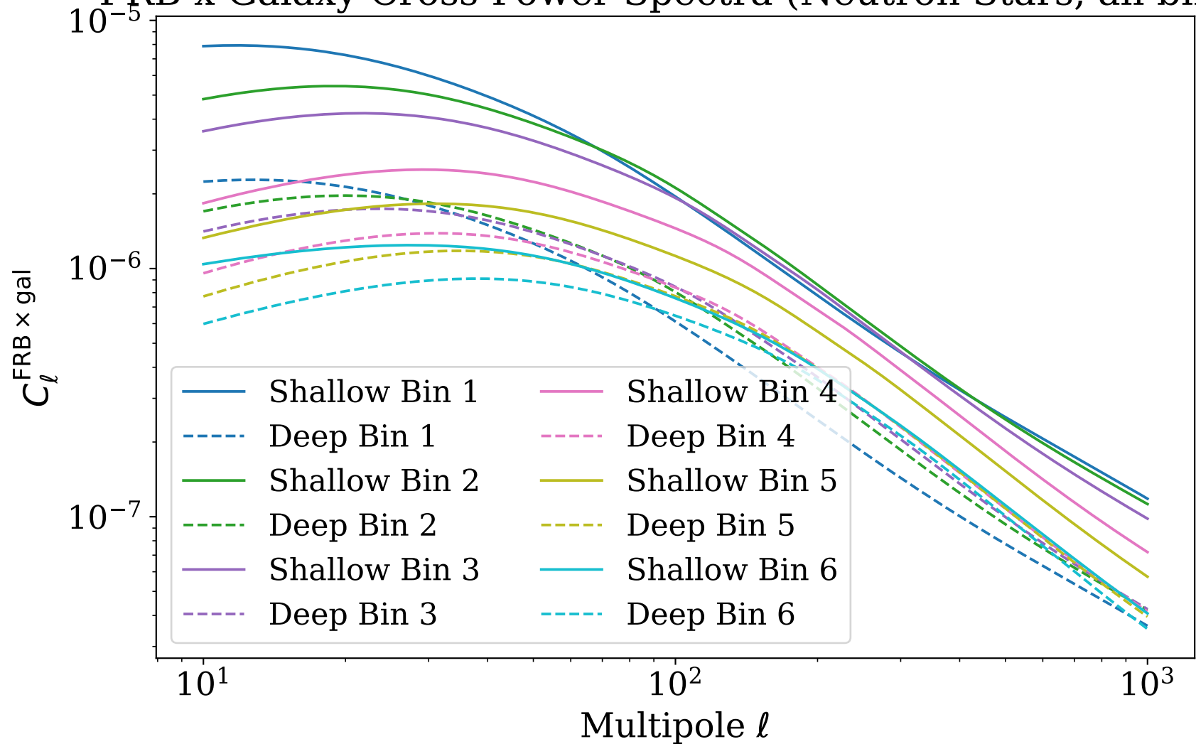
FRB x Galaxy Cross-Power Spectra (Neutron Stars, all bin
