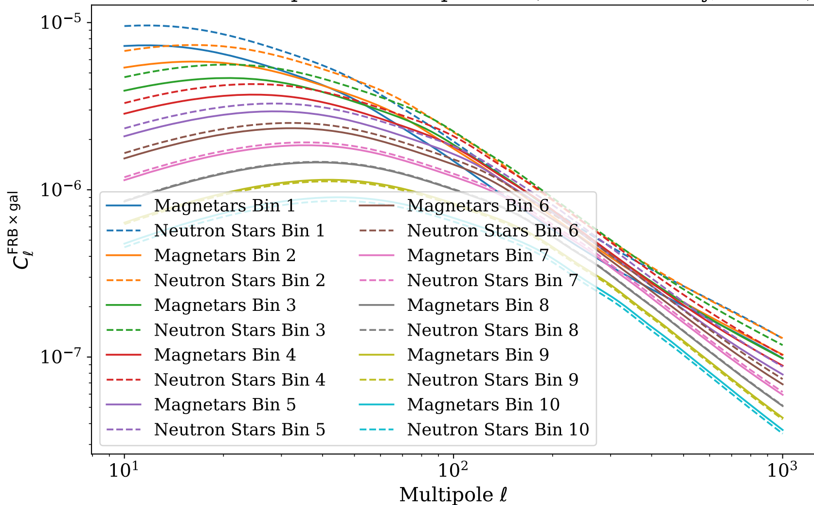
LSST Y10 FRB Population Comparison (Shallow Survey, all bins)
