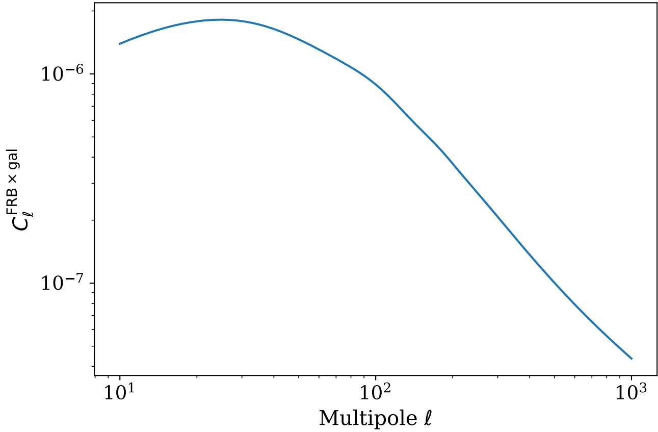
FRB×Galaxy Cross-Correlation (Neutron Stars, Deep Sur
