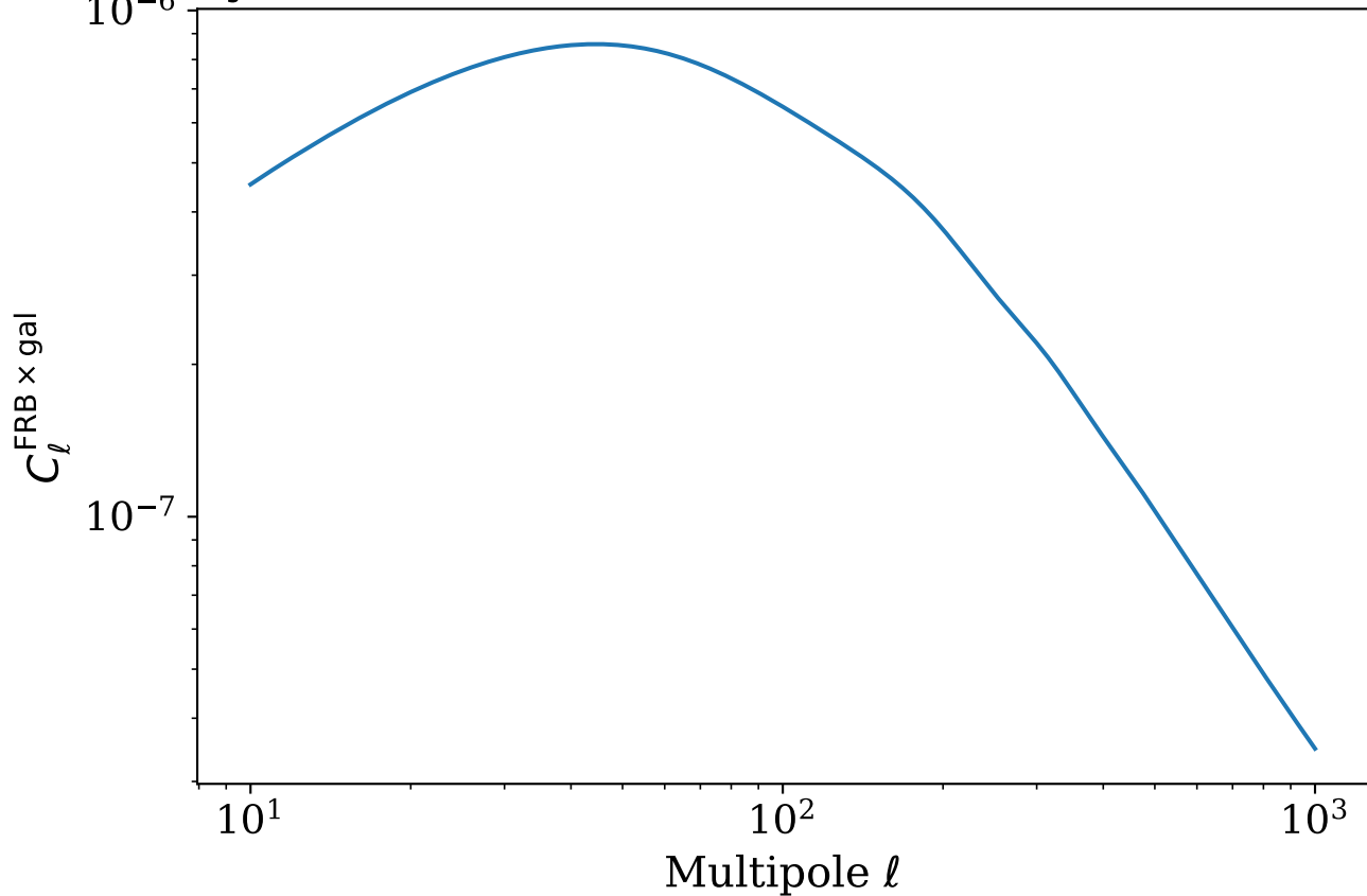
RB×Galaxy Cross-Correlation (Neutron Stars, Shallow Surveys)
