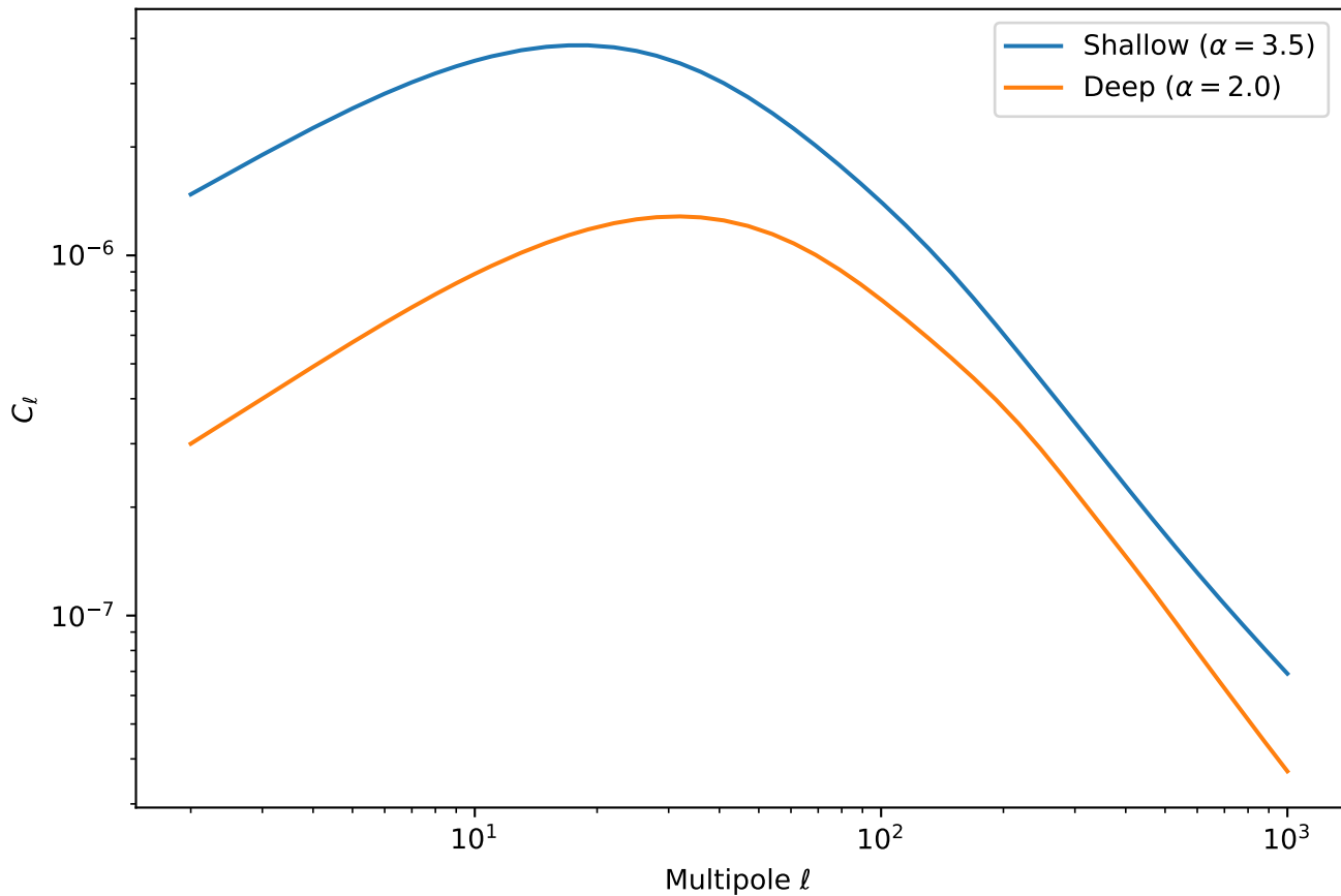
FRB Auto-Correlation: Shallow vs Deep Survey for Magnetars
