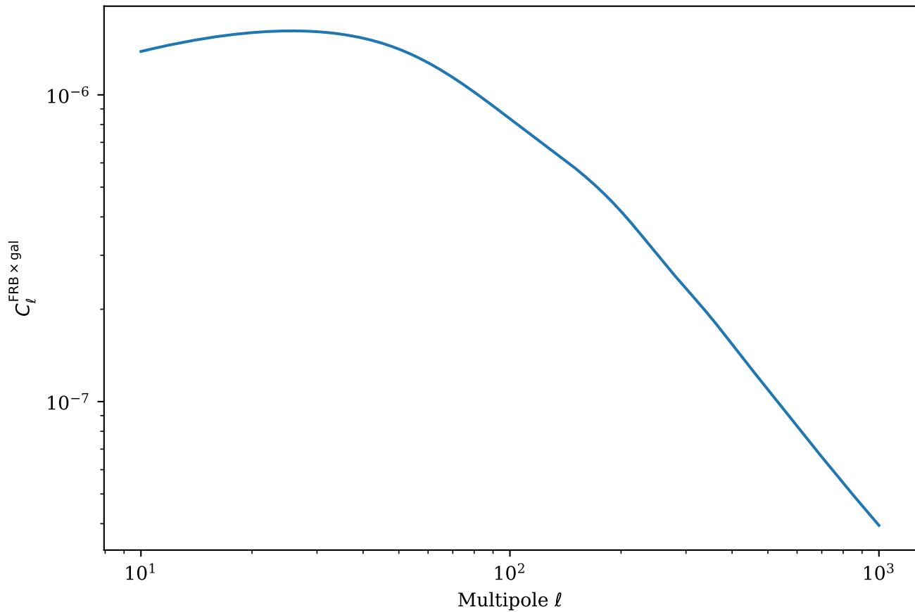
FRB×Galaxy Cross-Correlation (Neutron Stars, Shallow Survey, Galaxy Bin 0
