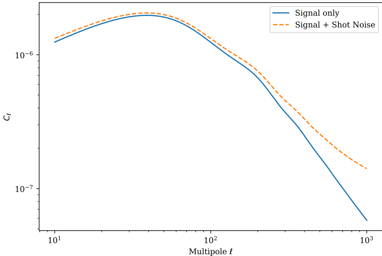
Galaxy Auto-Correlation Angular Power Spectrum (Bin 6 x Bin 6)
