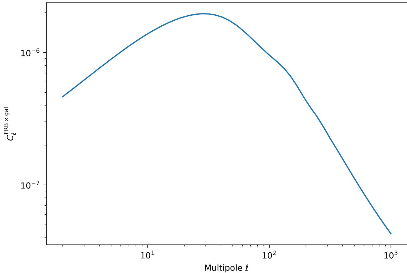
FRB×Galaxy Cross-Correlation (Neutron Stars, Deep Survey, Galaxy Bin 4)
