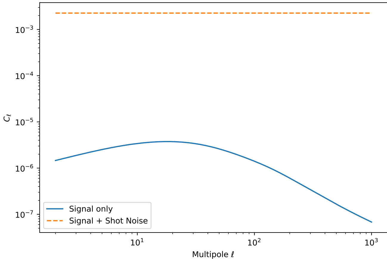
FRB Auto-Correlation Angular Power Spectrum (Shallow Survey) for Magnetar
