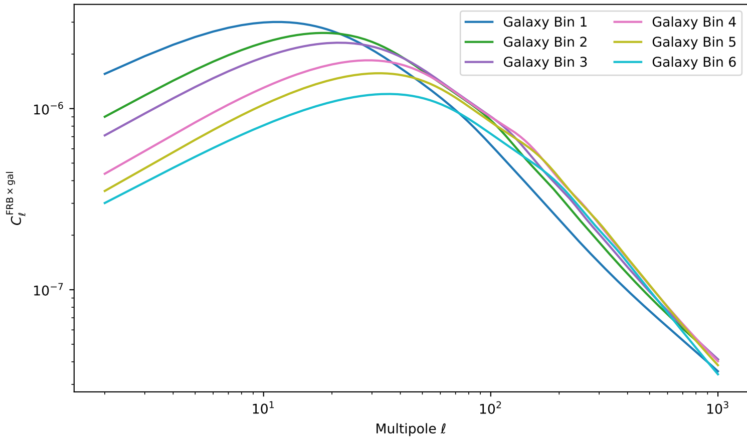
FRB×Galaxy — All Bins (Neutron Stars, Deep Survey)
