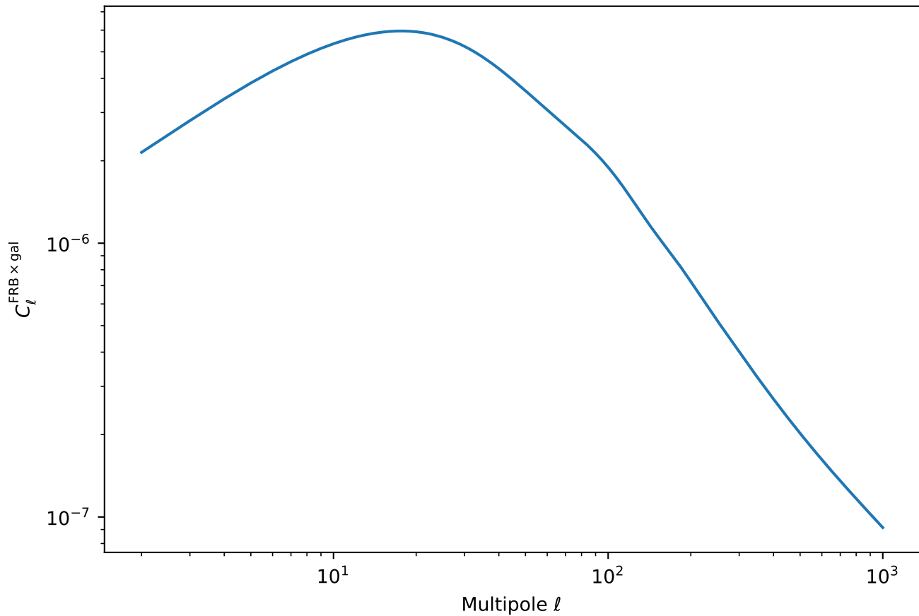
FRB×Galaxy Cross-Correlation (Magnetars, Shallow Survey, Galaxy Bin 2)
